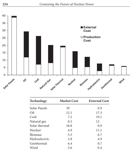
Figure 1: Production and External Costs for Electricity Generators (in US cents/kWh)
